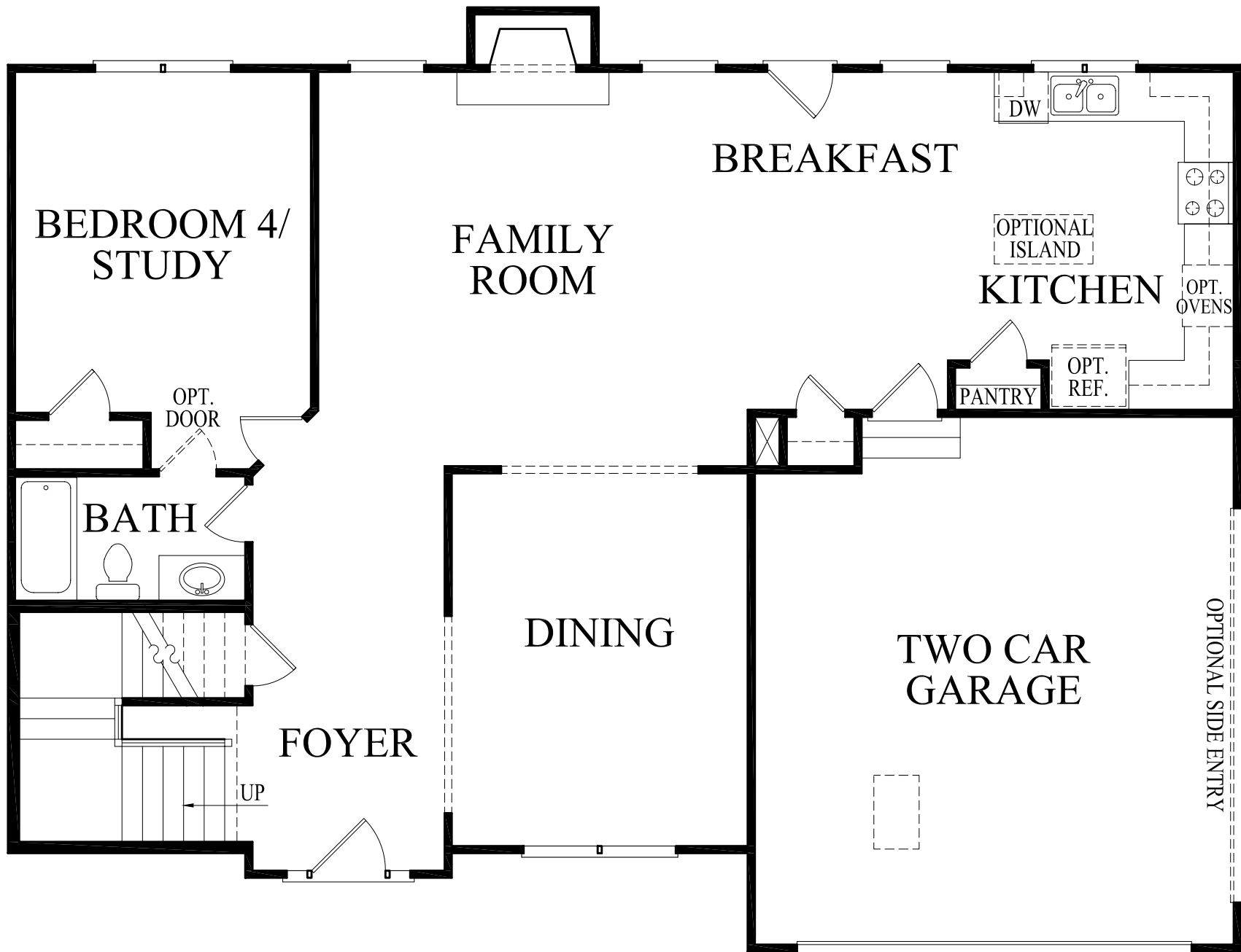
WESTMINSTER FIRST FLOOR 04-25-10
