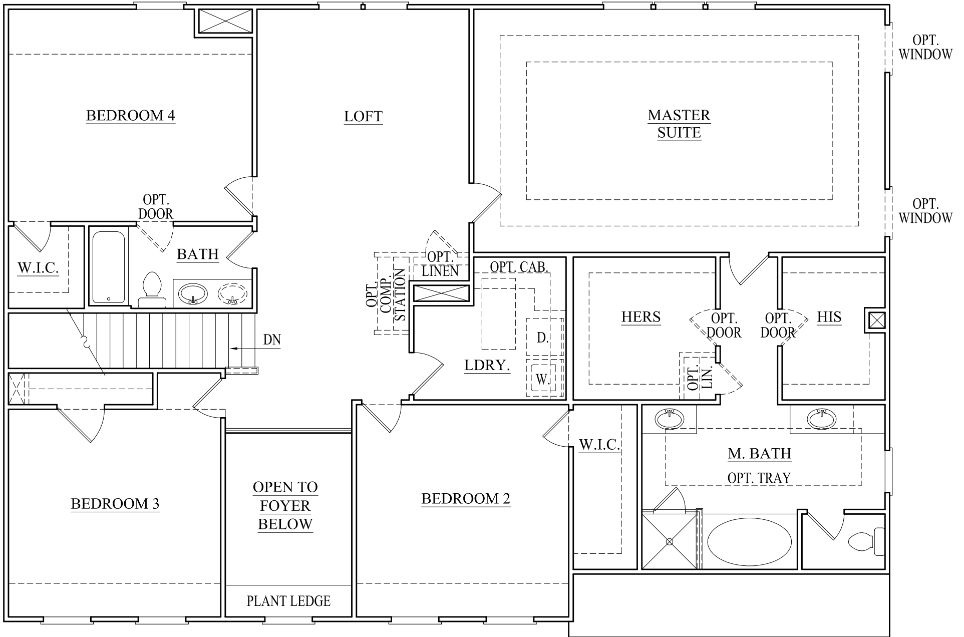
ARLINGTON SECOND FLOOR 02-04-08
